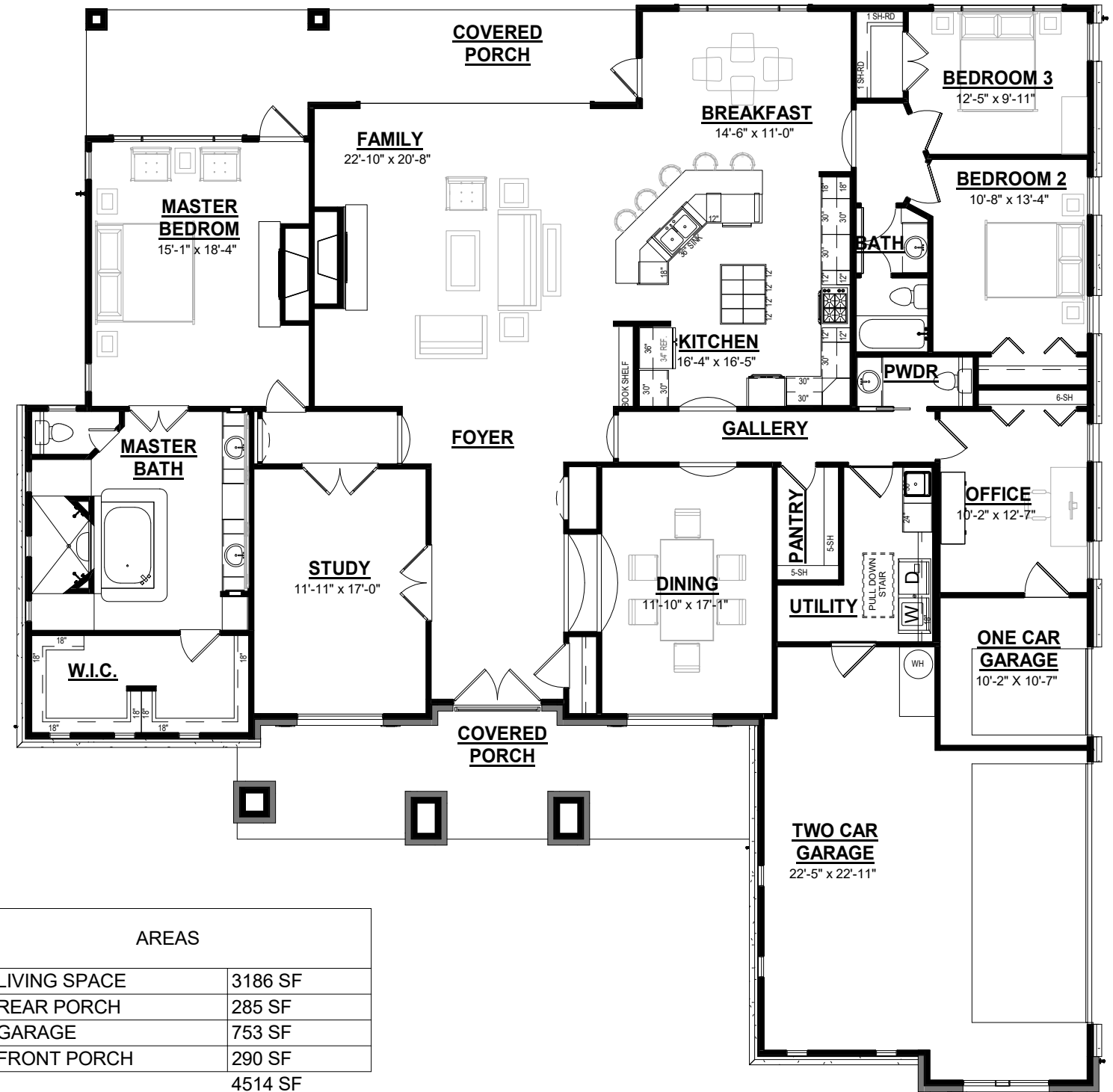
First Floor
